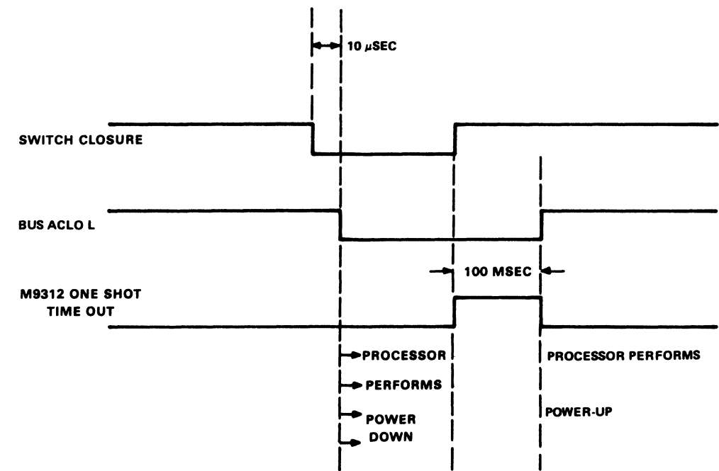
Figure 2-7 External Boot Timing
